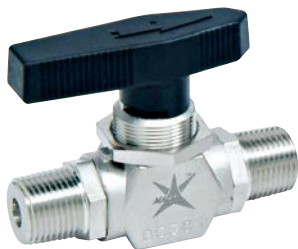
FIG. 200C 1/4" - 1/2", 3000 PSI Male/Female NPT or BSP
